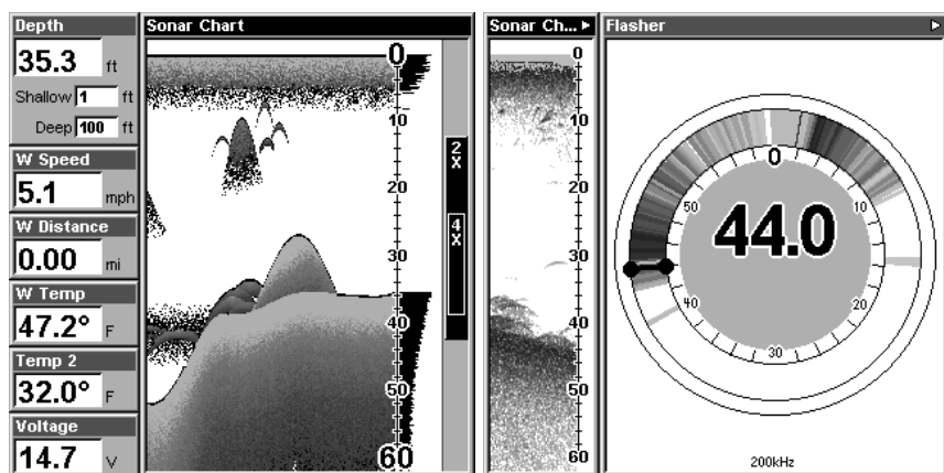
Sonar chart display options (from left) digital data and flasher.
