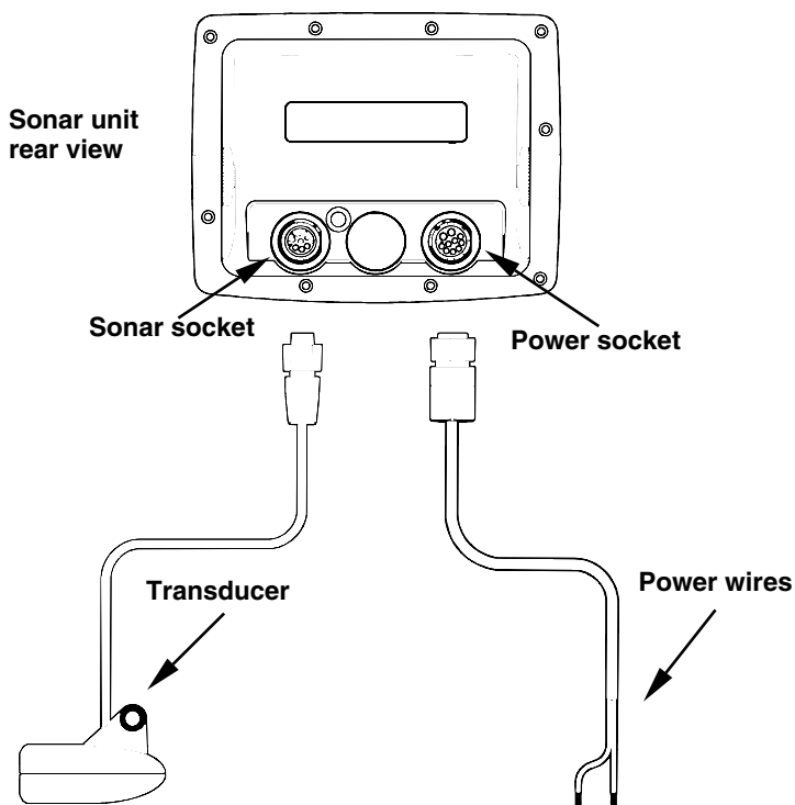
Sonar unit cable connections.
