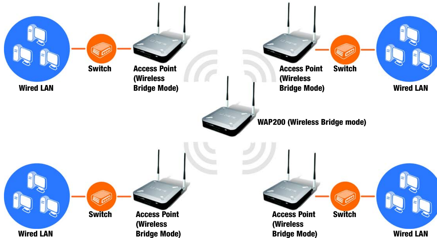
Figure 6-19: Wireless Bridge Mode
