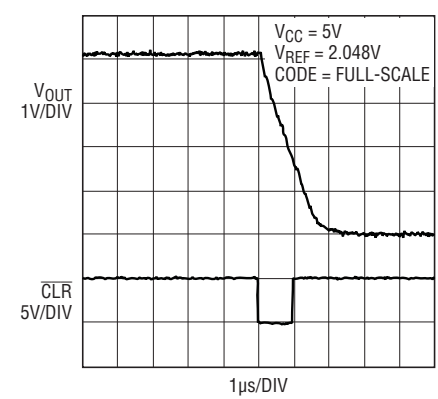
Hardware \overline{CLR} to Zero-Scale
