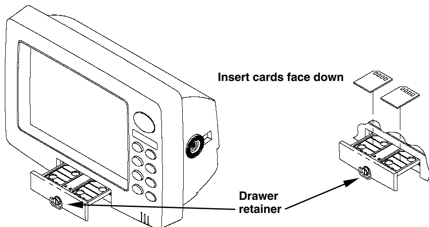
Memory card drawer on the GlobalMap 4000M.
