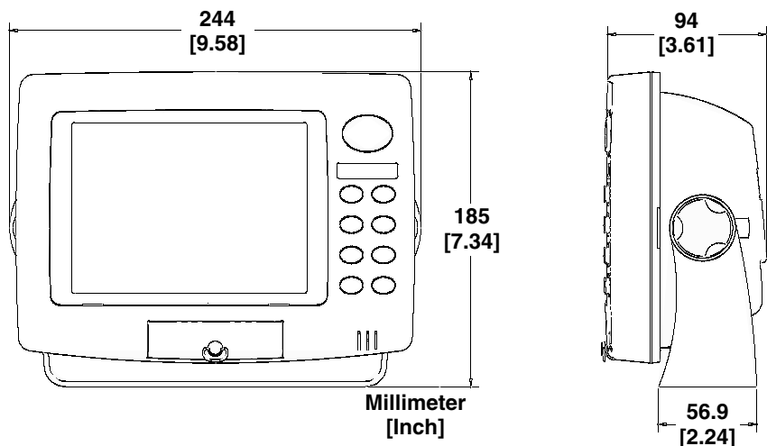
Front view (left) and side view (right) showing dimensions of the GlobalMap GPS unit when mounted on a gimbal bracket.
