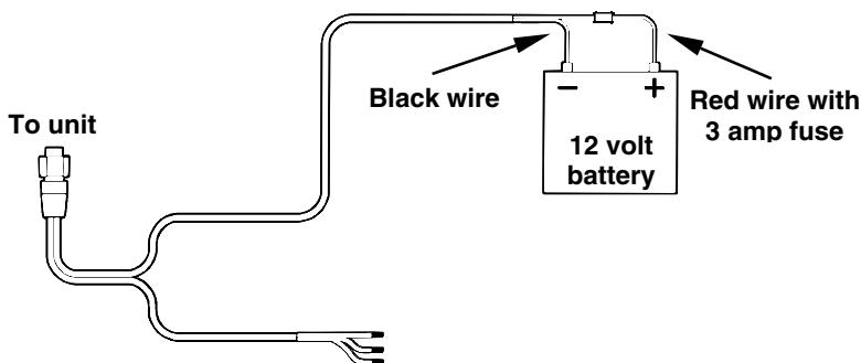
Power connections for the GlobalMap 4000M GPS unit.
