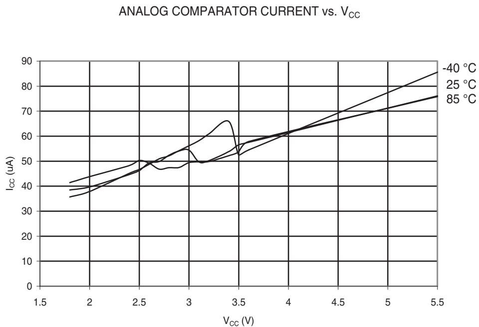
Figure 29-40. ATmega48PA: Analog Comparator Current vs. V_{CC} .
