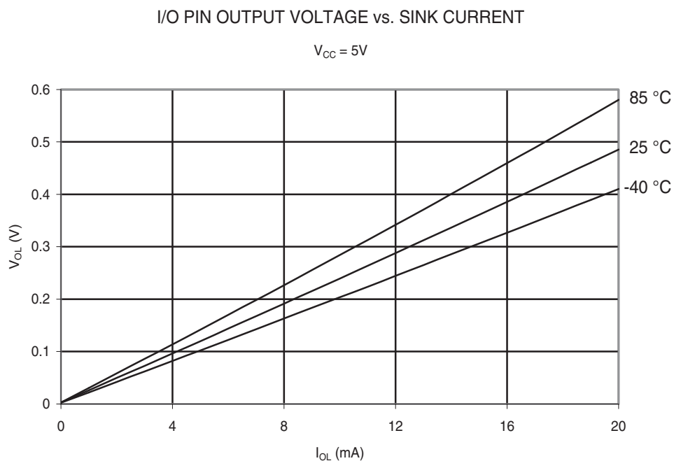
Figure 29-22. ATmega48PA: I/O Pin Output Voltage vs. Sink Current ( V_{CC} = 5\text{ V} ).
