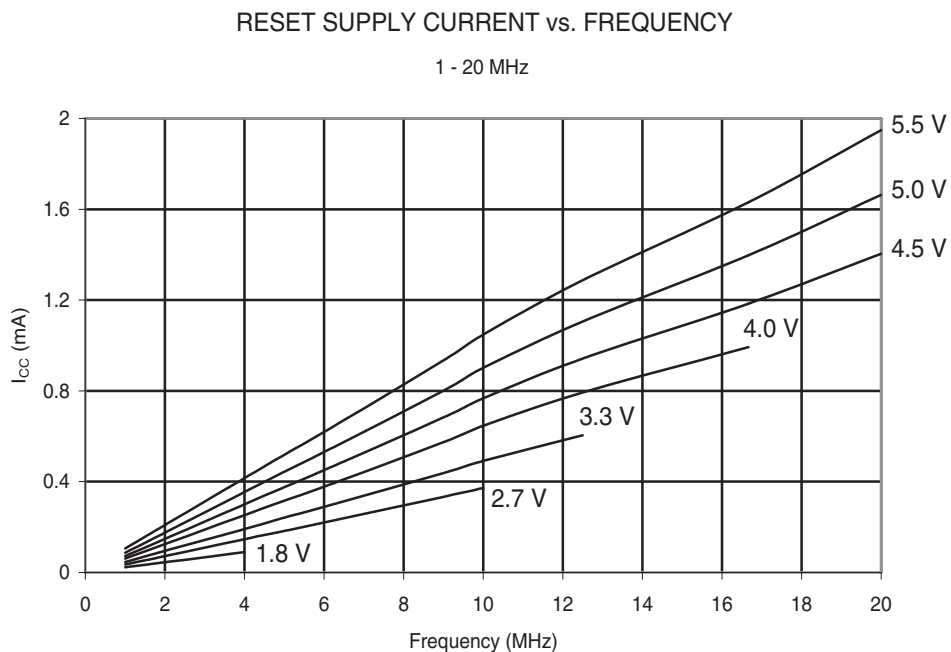
Figure 29-91. ATmega88PA: Reset Supply Current vs. Frequency (1 - 20 MHz).
