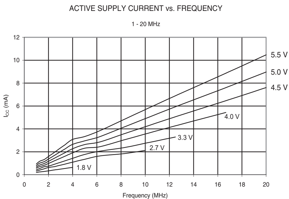
Figure 29-48. ATmega88PA: Active Supply Current vs. Frequency (1 - 20 MHz).
