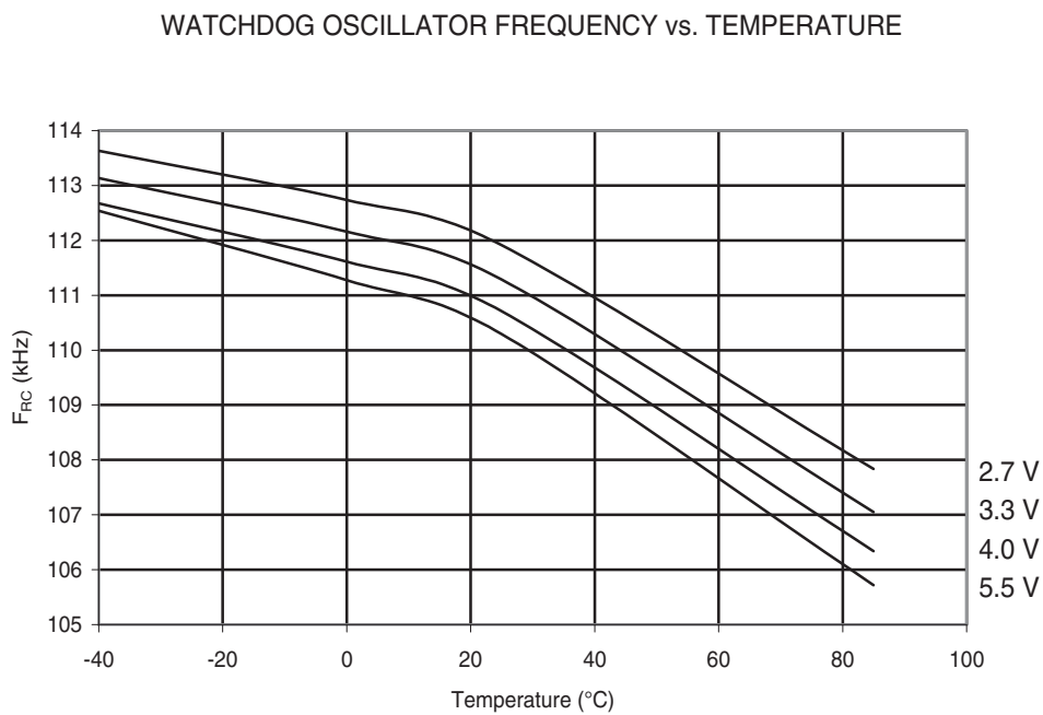
Figure 29-80. ATmega88PA: Watchdog Oscillator Frequency vs. Temperature.
