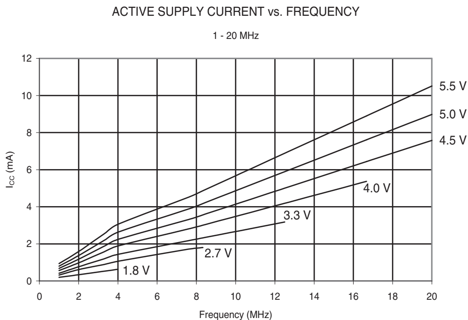
Figure 29-2. ATmega48PA: Active Supply Current vs. Frequency (1-20 MHz).
