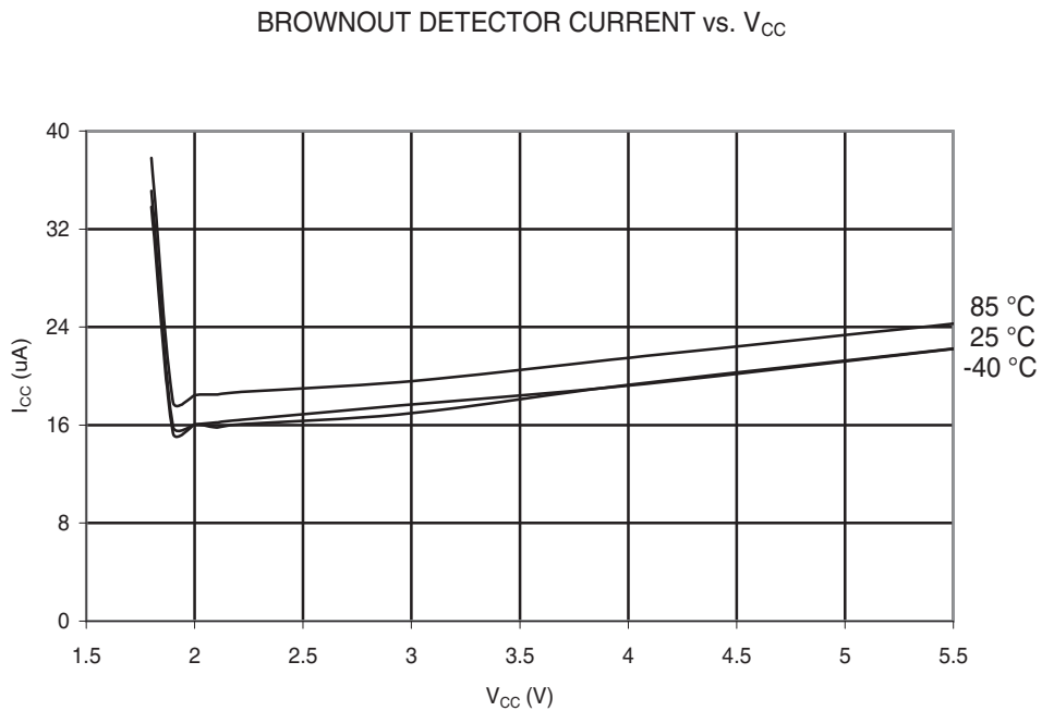
Figure 29-42. ATmega48PA: Brownout Detector Current vs. V_{CC} .
