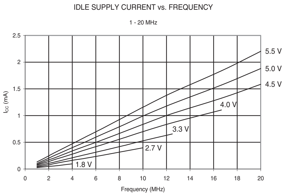
Figure 29-53. ATmega88PA: Idle Supply Current vs. Frequency (1 - 20 MHz).
