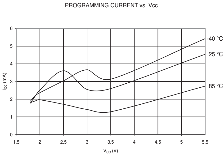
Figure 29-43. ATmega48PA: Programming Current vs. V_{CC} .
