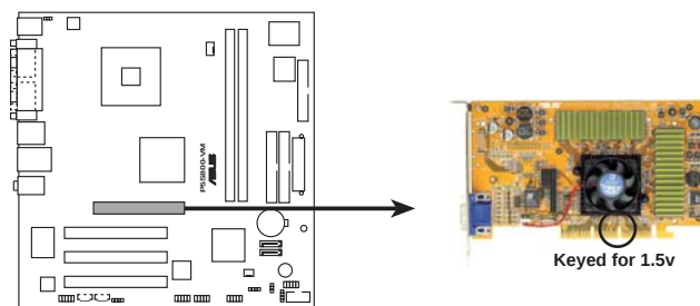
P5S800-VM Accelerated Graphics Port (AGP)
