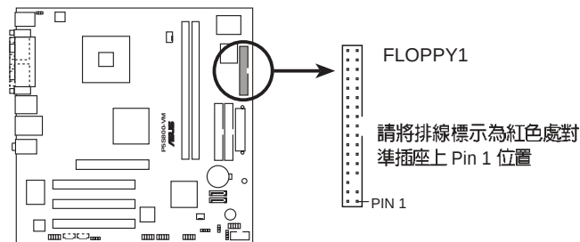
P5S800-VM Floppy disk drive connector
