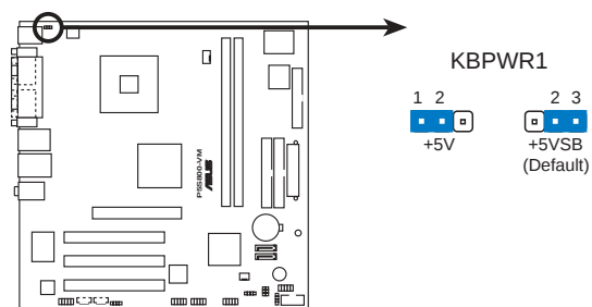
P5S800-VM Keyboard power setting
