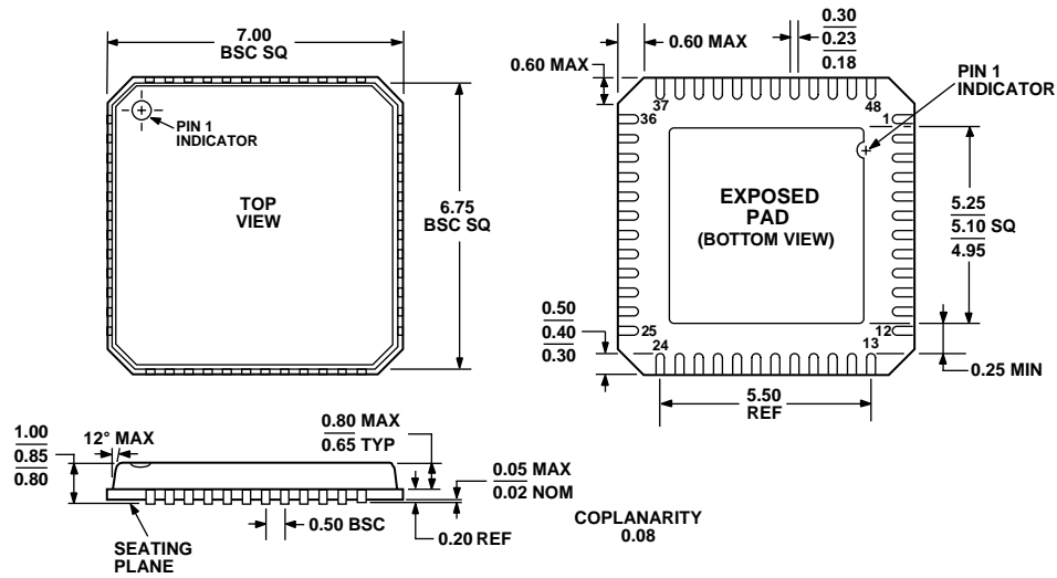
Figure 26. 48-Lead Frame Chip Scale Package [LFCSP] 7 mm x 7 mm Body (CP-48) Dimensions shown in millimeters
