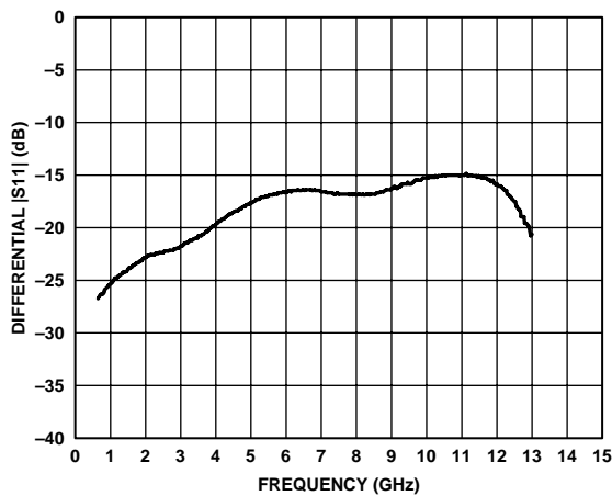
Figure 7. Differential |S_{11}|
