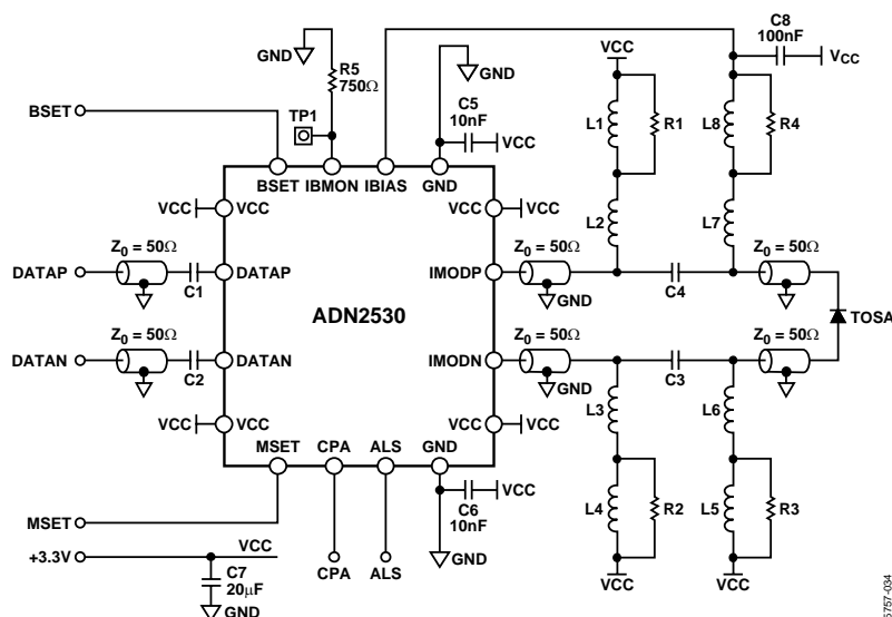
Figure 39. Typical ADN2530 Application Circuit
