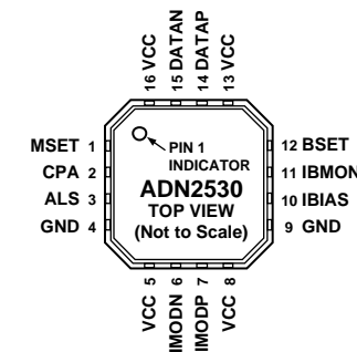
Figure 4. Pin Configuration
