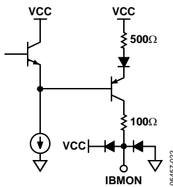
Figure 27. Equivalent Circuit of the IBMON Pin
