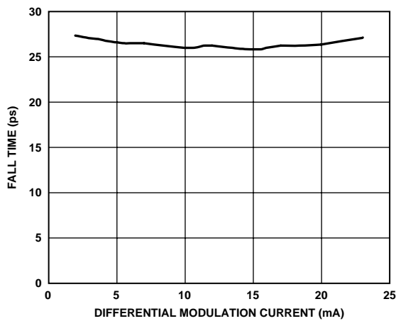
Figure 6. Fall Time vs. IMOD
