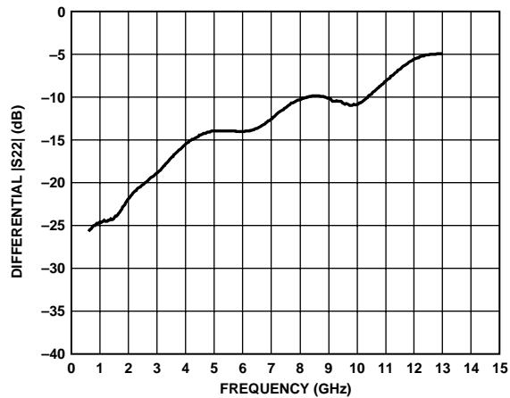
Figure 11. Differential |S_{22}|
