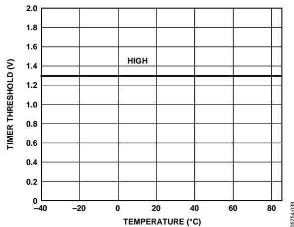
Figure 17. Timer Threshold vs. Temperature
