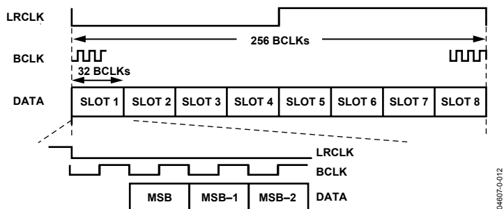
Figure 25. TDM Mode
