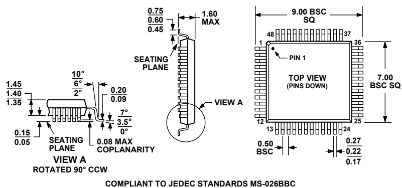
Figure 29. 48-Lead Low-Profile Quad Flat Package [LQFP] Dimensions Shown in Millimeters
