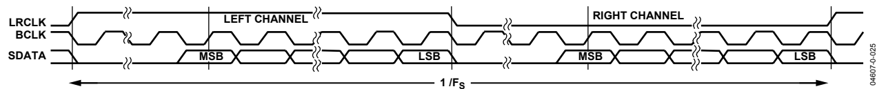
Figure 24. Right-Justified Mode—16 to 24 Bits per Channel
