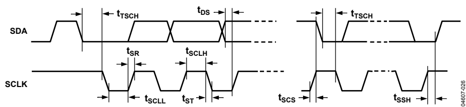
Figure 10. I²C Port Timing
