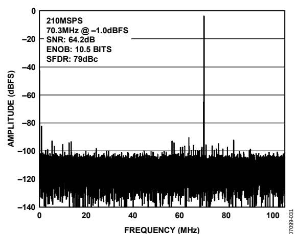
Figure 22. AD9626-210 64k Point Single-Tone FFT; 210 MSPS, 70.3 MHz
