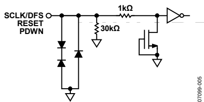
Figure 7. Equivalent SCLK/DFS, RESET, PDWN Input Circuit
