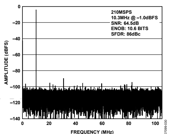
Figure 21. AD9626-210 64k Point Single-Tone FFT; 210 MSPS, 10.3 MHz
