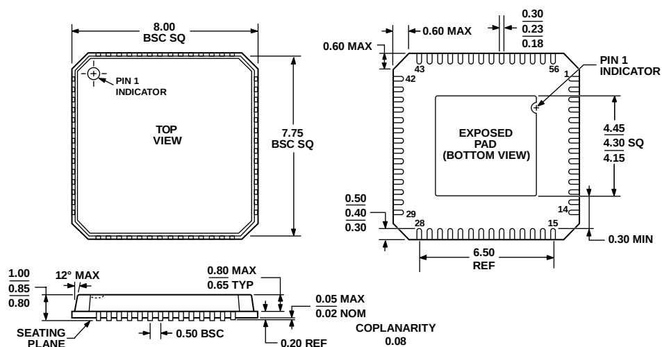
Figure 58. 56-Lead Lead Frame Chip Scale Package [LFCSP_VQ] 8 mm x 8 mm Body, Very Thin Quad (CP-56-2) Dimensions shown in millimeters
