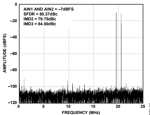
Figure 26. Two-Tone 32k FFT with f_{IN1} = 70 \text{ MHz} and f_{IN2} = 71 \text{ MHz} , f_{SAMPLE} = 50 \text{ MSPS}
