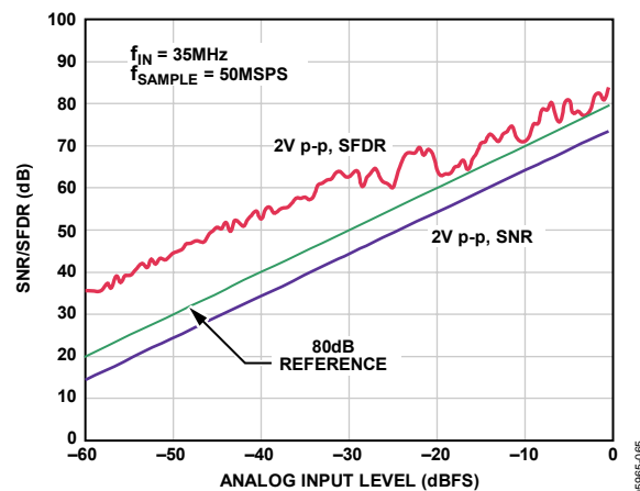
Figure 24. SNR/SFDR vs. Analog Input Level, f_{IN} = 35 \text{ MHz} , f_{SAMPLE} = 50 \text{ MSPS}
