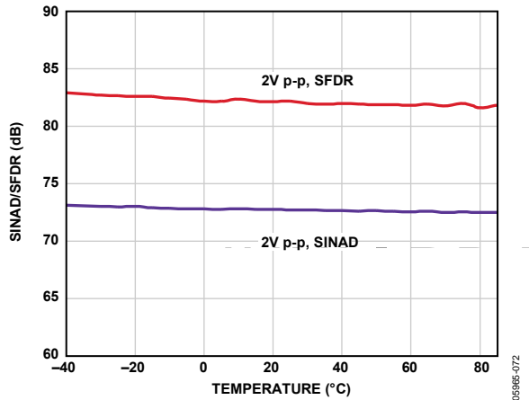
Figure 28. SINAD/SFDR vs. Temperature, f_{\text{IN}} = 10.3 \text{ MHz} , f_{\text{SAMPLE}} = 50 \text{ MSPS}
