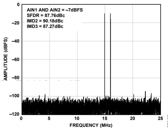
Figure 25. Two-Tone 32k FFT with f_{IN1} = 15 \text{ MHz} and f_{IN2} = 16 \text{ MHz} , f_{SAMPLE} = 50 \text{ MSPS}
