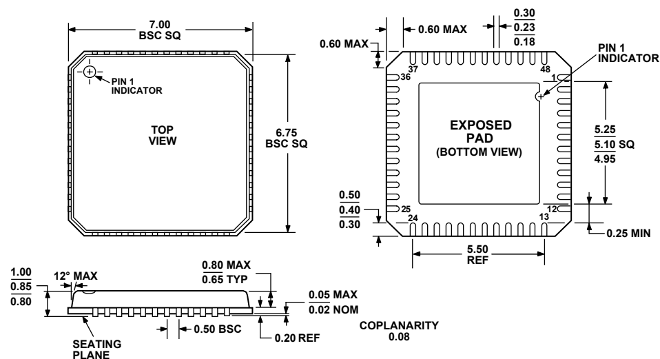
Figure 71. 48-Lead Lead Frame Chip Scale Package [LFCSP_VQ]
