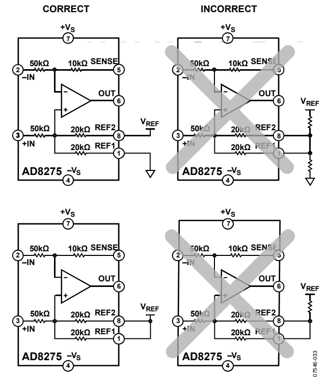
Figure 35. REF1 and REF2 Pin Guidelines
