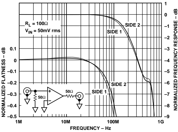
Figure 6. Frequency Response and Flatness
