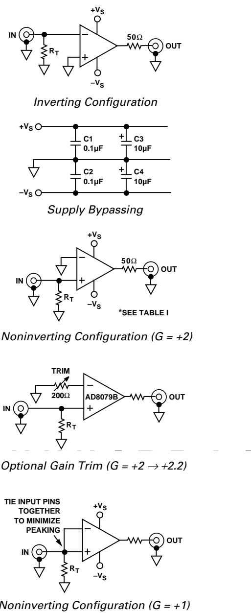
Figure 29. Inverting and Noninverting Configurations
