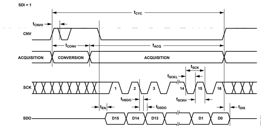
Figure 35. \overline{\text{CS}} Mode, 3-Wire Without Busy Indicator Serial Interface Timing (SDI High)
