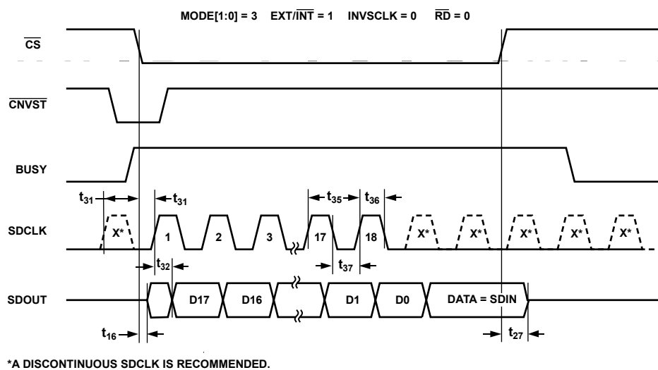
Figure 45. Slave Serial Data Timing for Reading (Read Previous Conversion During Convert)
