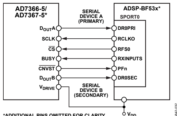
Figure 30. Interfacing the AD7366-5/AD7367-5 to the ADSP-BF53x
