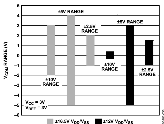
Figure 38. Common-Mode Range for V_{CC} = 3V and REF_{IN}/REF_{OUT} = 3V
