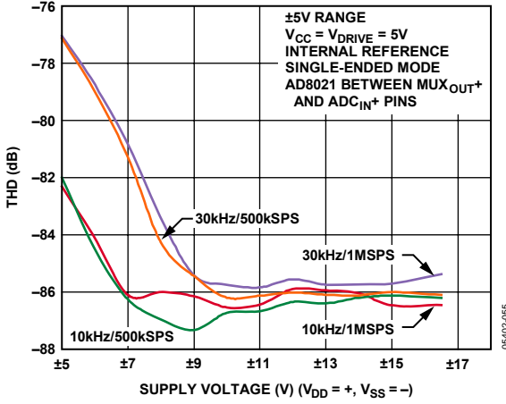
Figure 23. THD vs. Supply Voltage at 500 kSPS and 1 MSPS with 10 kHz and 30 kHz Input Tone
