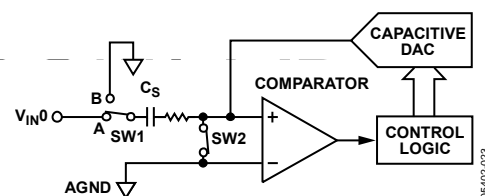
Figure 24. ADC Acquisition Phase (Single Ended)
