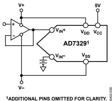
Figure 42. Pseudo Differential Inputs
