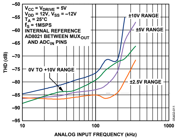
Figure 11. THD vs. Analog Input Frequency for True Differential Mode (Diff) at 5 V V_{CC}
