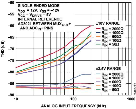
Figure 22. THD vs. Analog Input Frequency for Various Source Impedances, Single-Ended Mode
