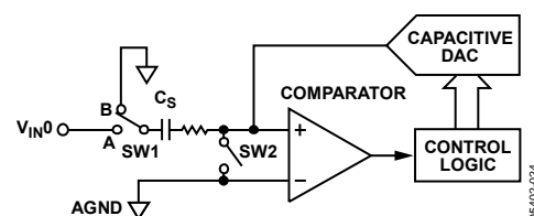
Figure 25. ADC Conversion Phase (Single Ended)
