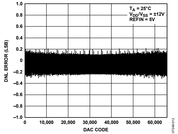
Figure 10. Differential Nonlinearity Error vs. DAC Code, V_{DD}/V_{SS} = \pm 12\text{ V}
