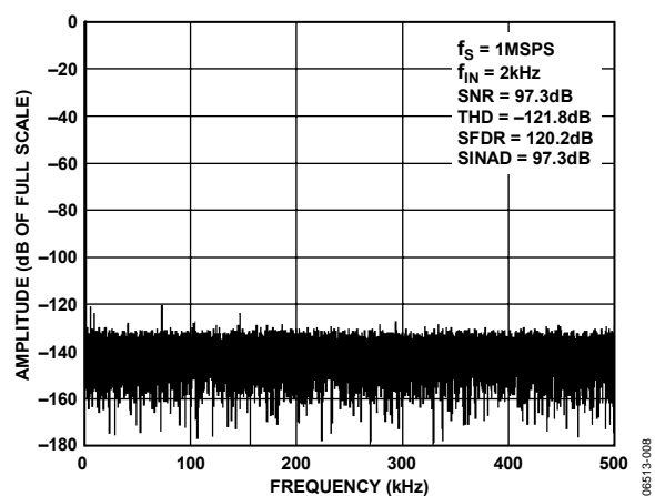
Figure 8. FFT Plot
