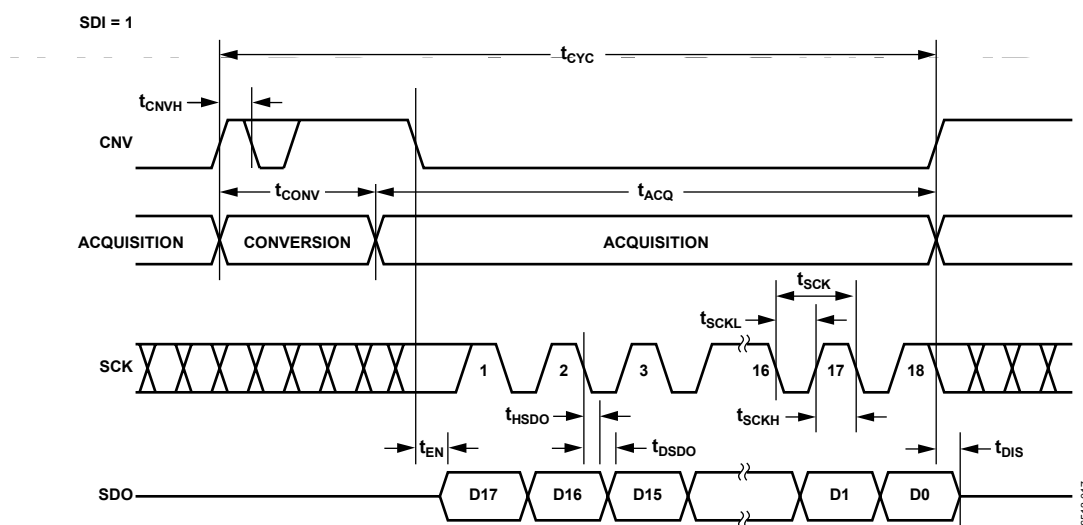
Figure 30. \overline{\text{CS}} Mode, 3-Wire Without Busy Indicator Serial Interface Timing (SDI High)
