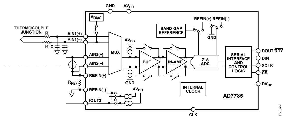
Figure 20. Thermocouple Measurement Using the AD7785
