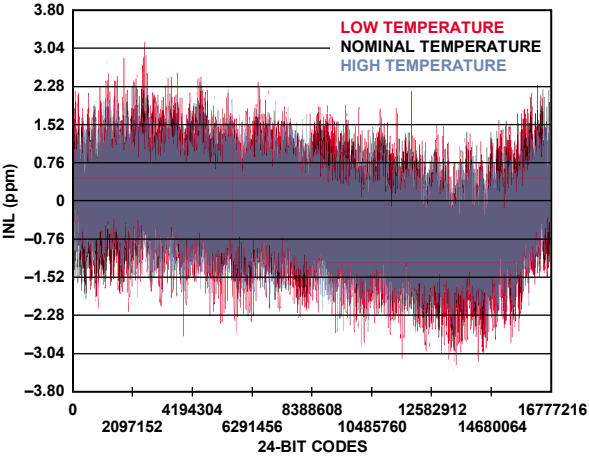
Figure 27. AD7767/AD7767-1/AD7767-2, 24-Bit INL
