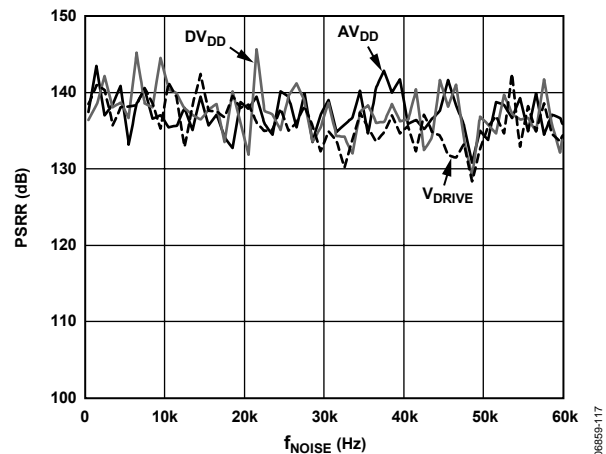
Figure 21. AD7767 Power Supply Sensitivity vs. Supply Ripple Frequency with Decoupling Capacitors
