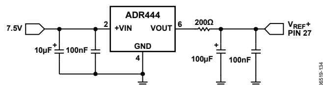
Figure 41. Reference Connection
