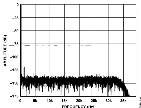
Figure 10. Low Power Mode; FFT, 1 kHz, -0.5\text{ dB} Input Tone, 256 \times Decimation Rate
