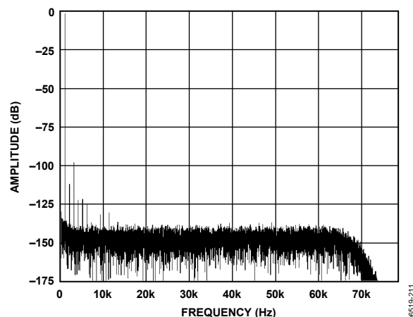
Figure 9. Low Power Mode; FFT, 1 kHz, -0.5\text{ dB} Input Tone, 128 \times Decimation Rate
