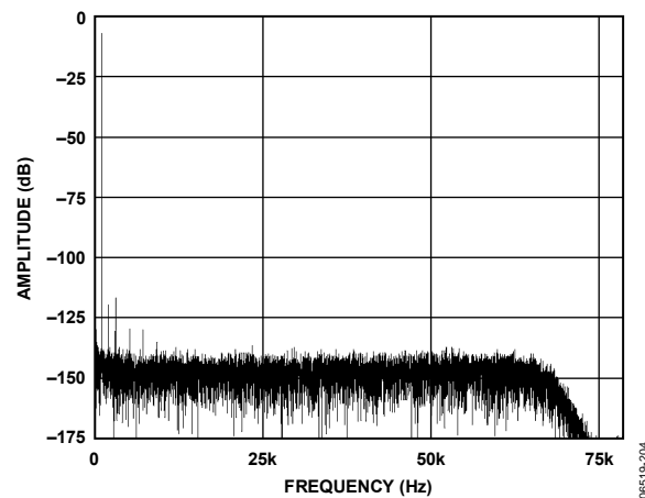
Figure 11. Low Power Mode; FFT, 1 kHz, - \text{dB} Input Tone, 128 \times Decimation Rate
