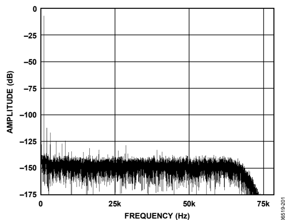
Figure 8. Normal Power Mode; FFT, 1 kHz, -6\text{ dB} Input Tone, 128 \times Decimation Rate
