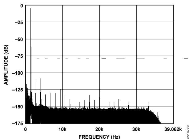
Figure 7. Normal Power Mode; FFT, 1 kHz, -0.5\text{ dB} Input Tone, 256 \times Decimation Rate
