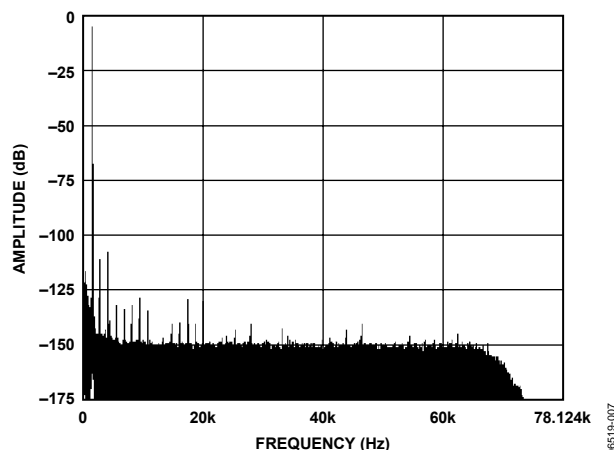
Figure 6. Normal Power Mode; FFT, 1 kHz, -0.5\text{ dB} Input Tone, 128 \times Decimation Rate
