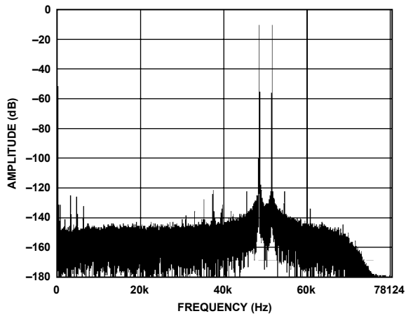
Figure 19. Normal Power Mode; IMD, f_{IN A} = 49.7 kHz, f_{IN B} = 50.3 kHz, 50 kHz Center Frequency, 128× Decimation Rate
