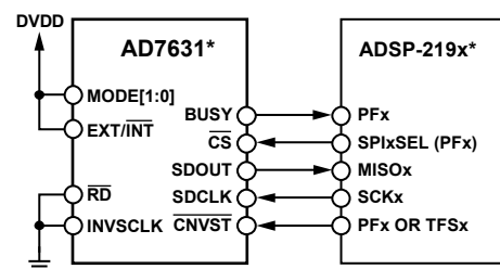
Figure 48. Interfacing the AD7631 to SPI Interface
