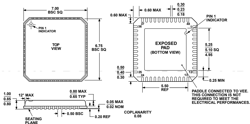
Figure 50. 48-Lead Lead Frame Chip Scale Package [LFCSP_VQ] 7 mm x 7 mm Body, Very Thin Quad (CP-48-1)
