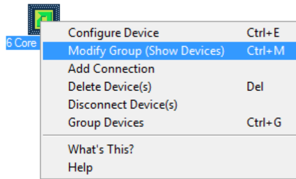
Figure 3-9: Modify Group
