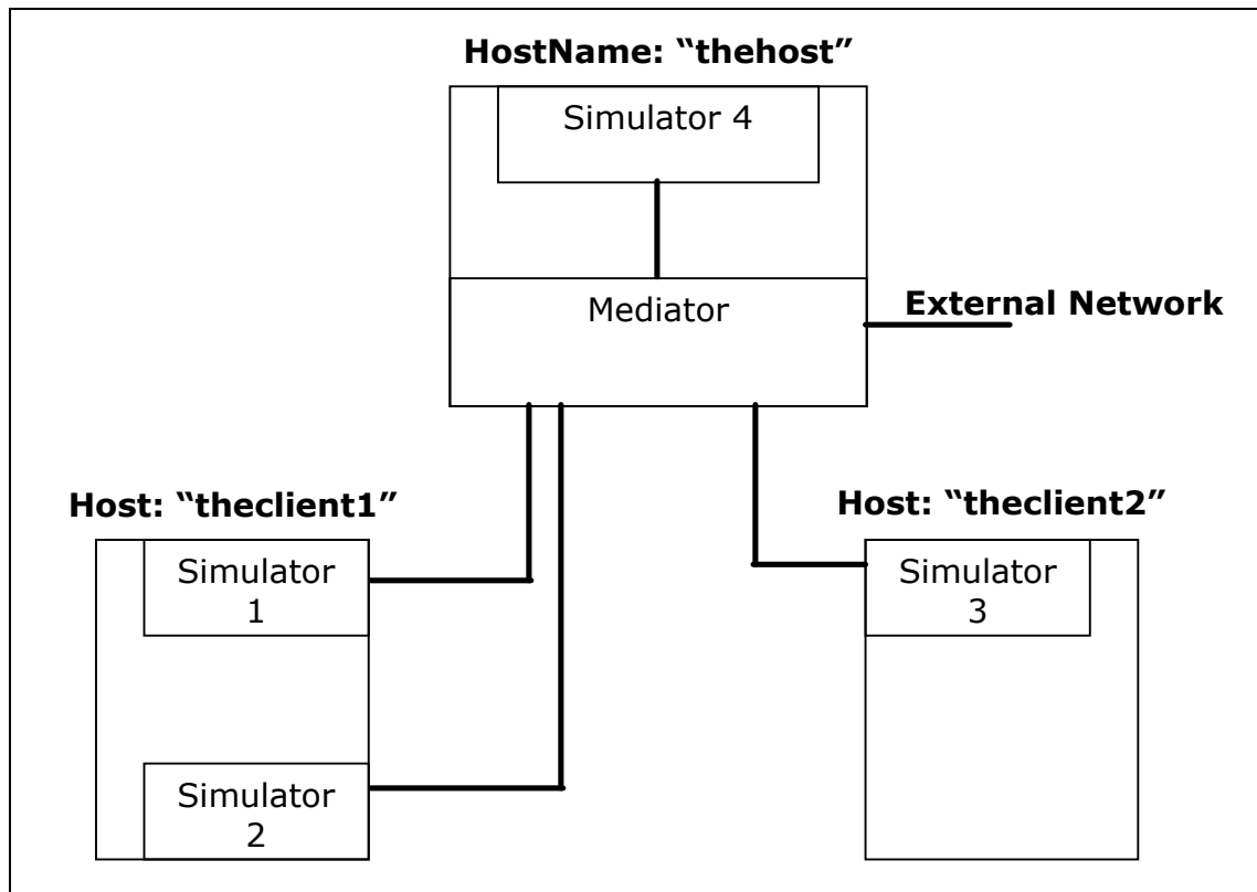
Figure 7-35: Communication via Mediator
