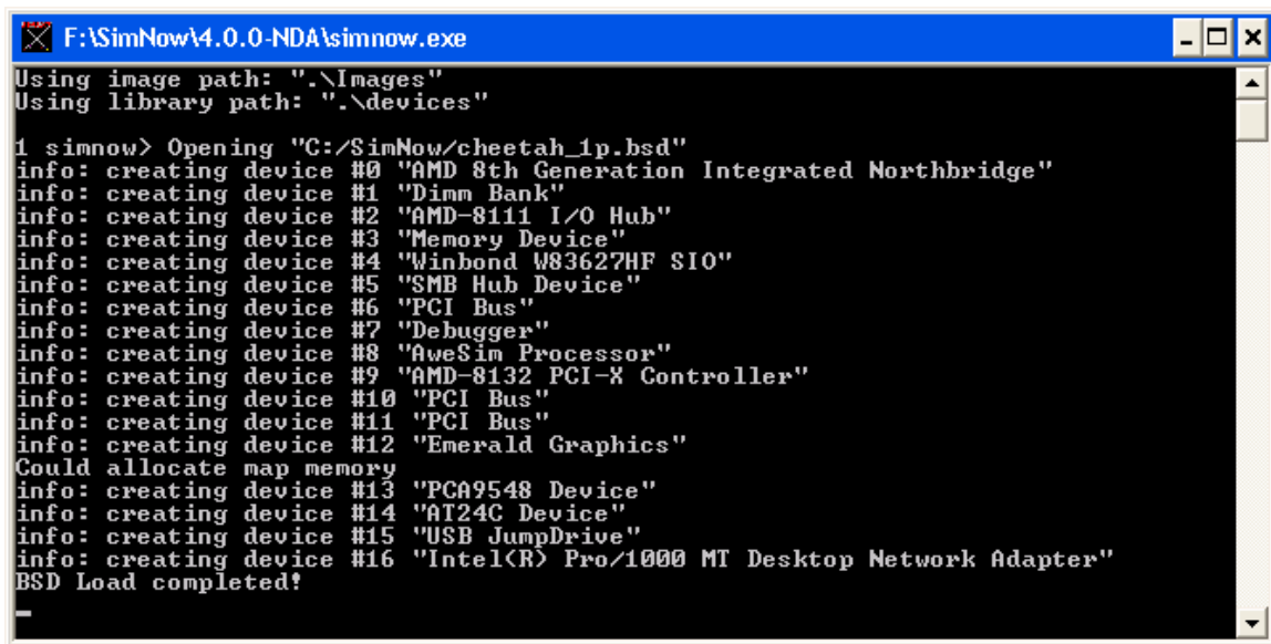
Figure 3-15: Console Window
