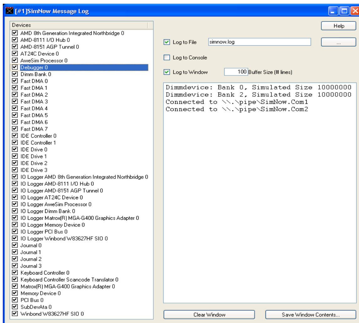
Figure 9-1: Message Log
