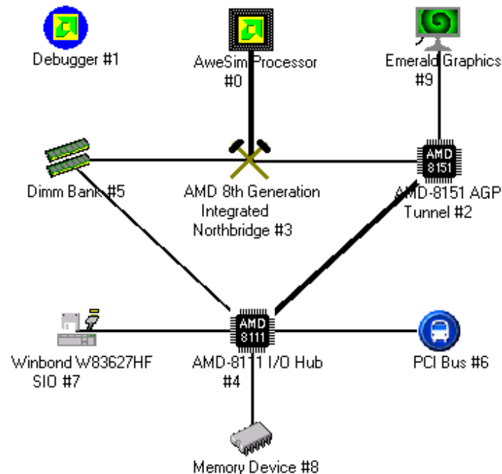
Figure 6-1: Solo.bsd Configuration
