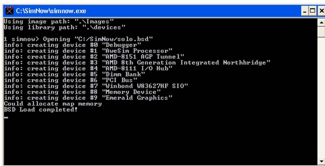
Figure 15-1: Console Window
