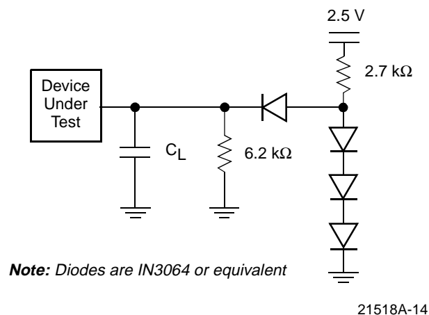
Figure 12. Test Setup
