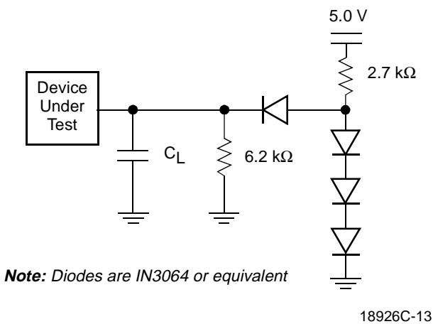
Figure 8. Test Setup
