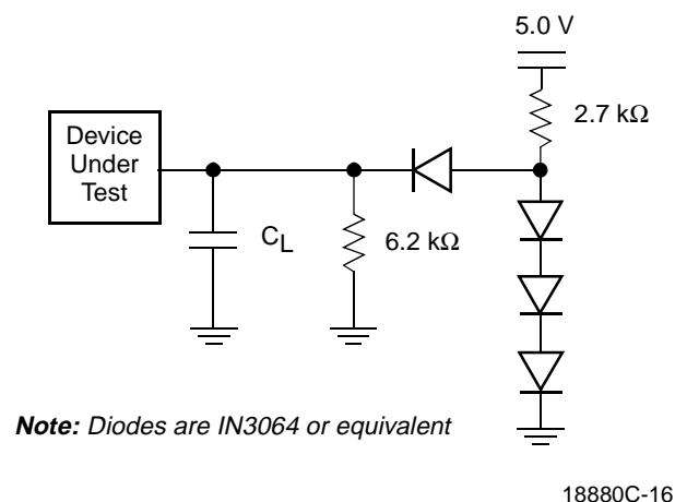
Figure 8. Test Setup
