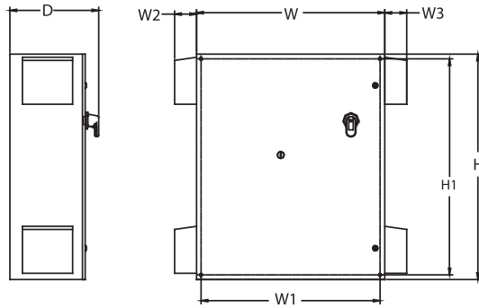
CX3R-1 to CX3R-9 Wall Mounted
