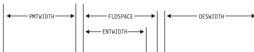
Figure 108. PMTWIDTH, ENTWIDTH, FLDSpace, and DESWIDTH attributes
