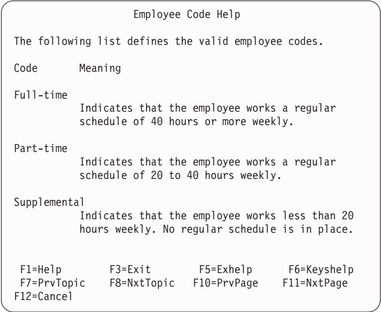
Figure 105. Definition List (BREAK=ALL)
