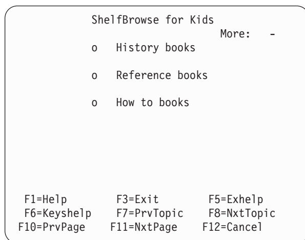
Figure 122. Help panel (example 3 of 3)
