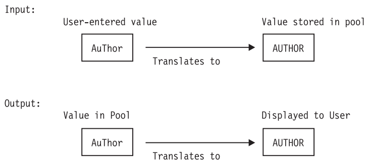
Figure 24. Variable translation results
