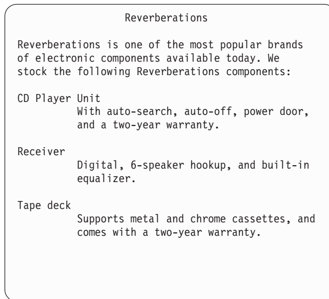
Figure 56. Definition list ( BREAK=ALL )
