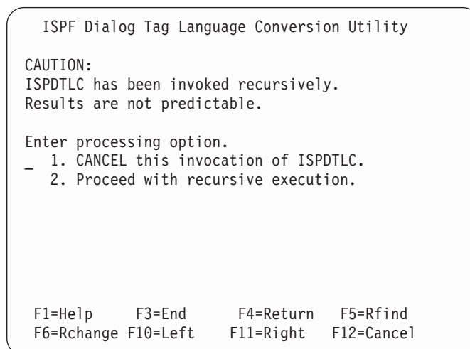
Figure 84. ISPF Dialog Tag Language conversion utility - recursive invoke
