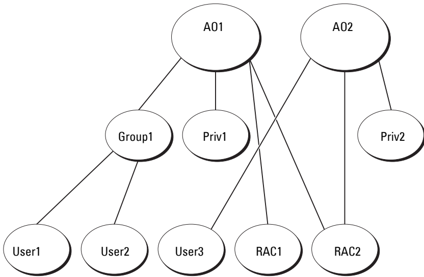
Figure 9-2. Setting Up Active Directory Objects in a Single Domain
