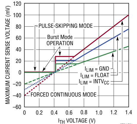
Maximum Current Sense Threshold vs I TH Voltage
