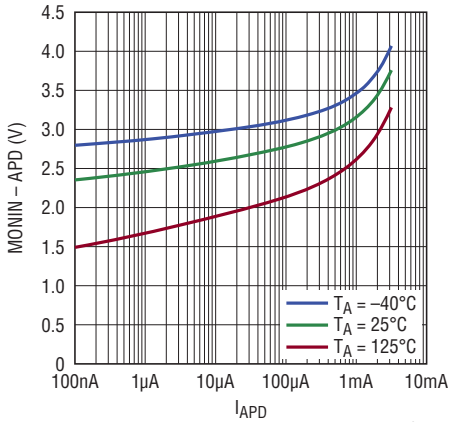
Current Monitor Voltage Drop vs APD Current
