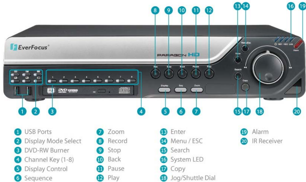
Figure 1-1 Front Panel
