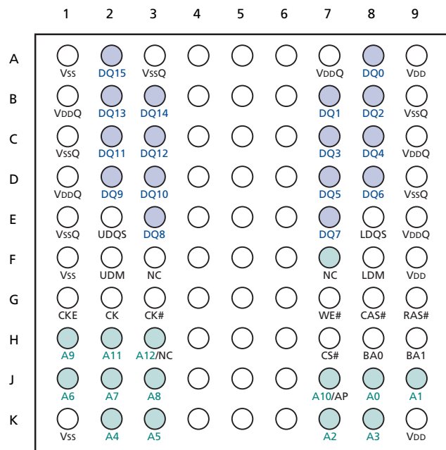
Figure 1: 60-Ball VFBGA Assignment (Top View)
