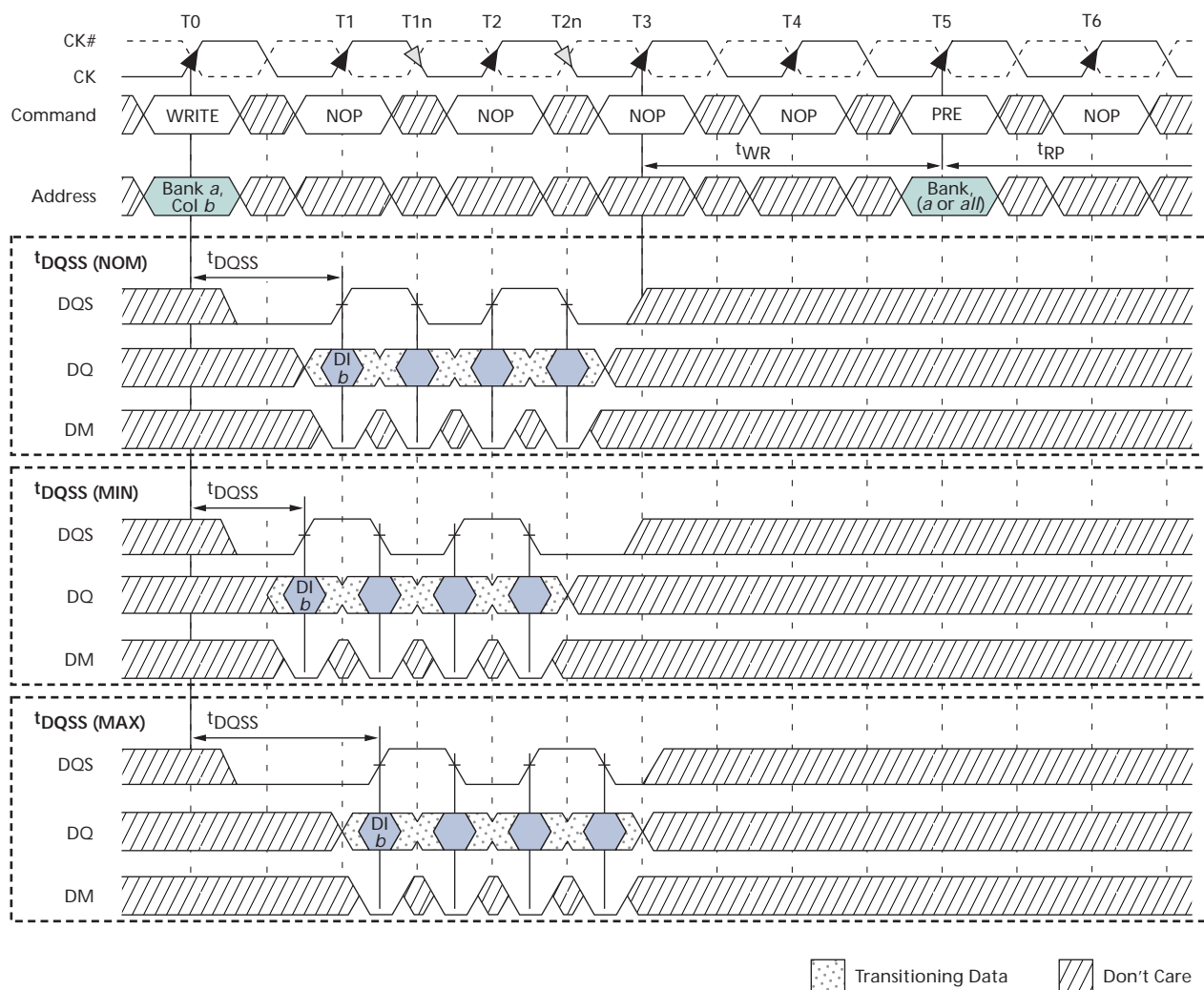
Figure 43: WRITE-to-PRECHARGE – Uninterrupting
