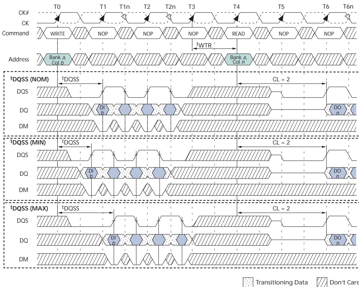
Figure 40: WRITE-to-READ – Uninterrupting
