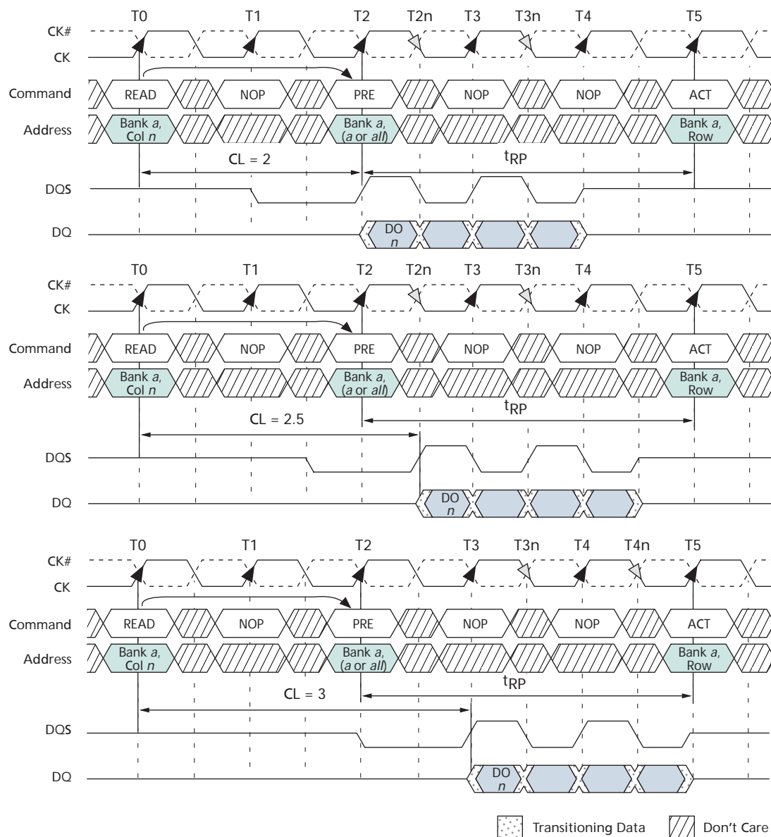
Figure 31: READ-to-PRECHARGE
