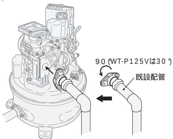
[取付例：WT-P200V]
