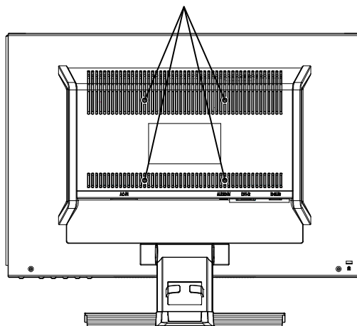
螺丝孔 (75 mm x 75 mm)
