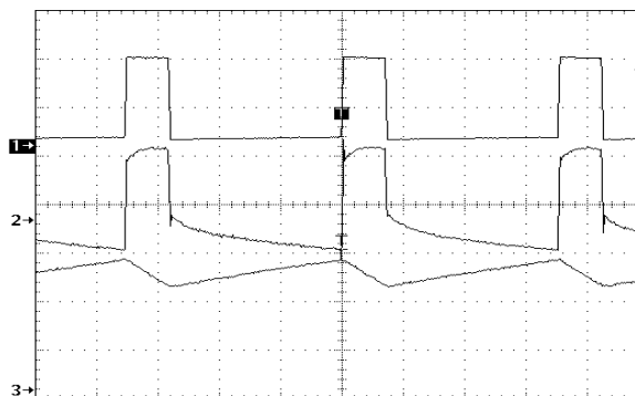
Figure 40. NCP1402SN19T1 Operating Waveforms (Heavy Load)
