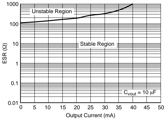
Figure 2. Output Stability
