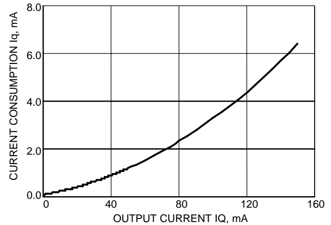
Figure 13. Current Consumption I_q vs. Output Current I_Q
