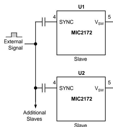
Figure 7. External Synchronization
