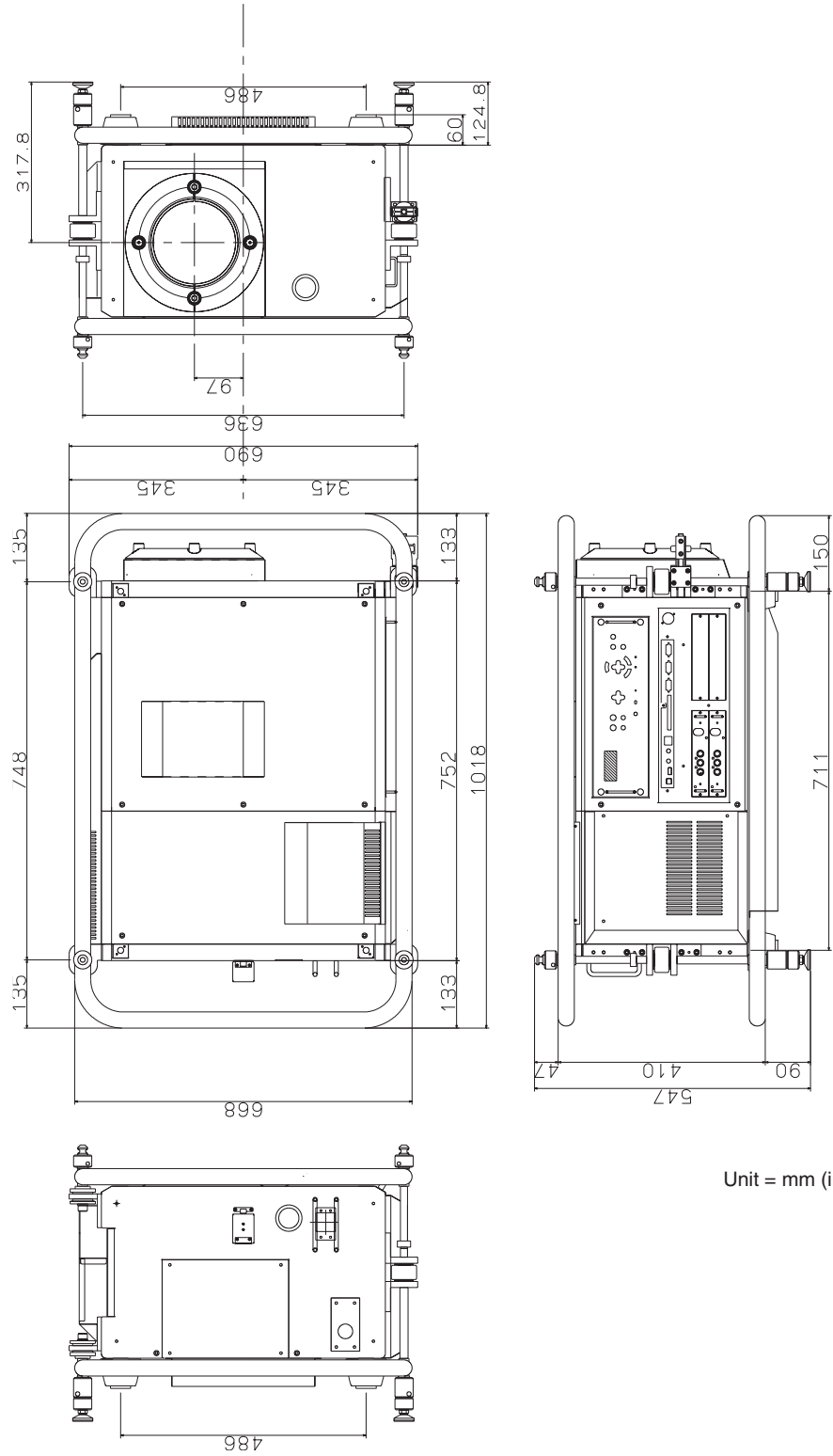
HIGHlite 14000HD
