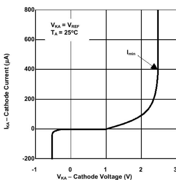
Cathode Current vs. Cathode Voltage
