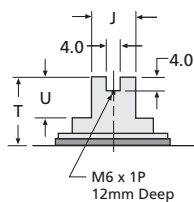
NAMUR SOLENOID MOUNTING
