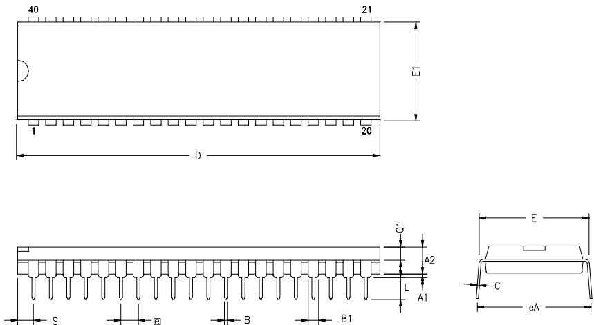
Figure 38. 40-Pin PDIP
