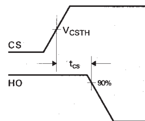
Figure 4. CS Shutdown Waveform Definitions
