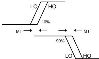
Figure 4. Deadtime Waveform Definitions
