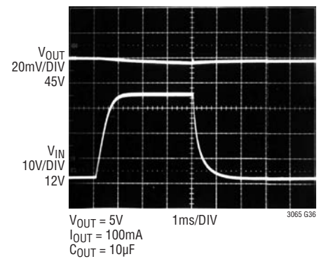
Transient Response (Load Dump)
