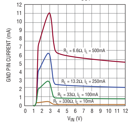
GND Pin Current, V_{OUT} = 3.3\text{V}
