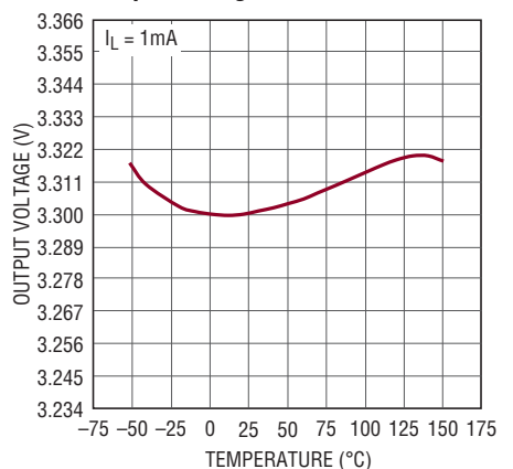
Output Voltage = 3.3V
